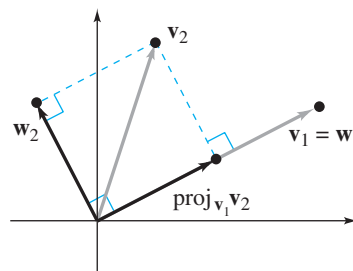
\mathbf{w}_2 = \mathbf{v}_2 - \text{proj}_{\mathbf{v}_1} \mathbf{v}_2 is orthogonal to \mathbf{w}_1 = \mathbf{v}_1 .
